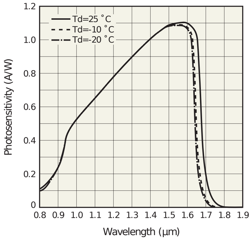
Figure 1: Photosensitivity of the Hamamatsu G12180 InGaAs-Photodiode. Source: Hamamatsu Photonics K.K., "InGaAs PIN photodiodes G12180 series", G12180-005 datasheet, Jan. 2021, page 3
