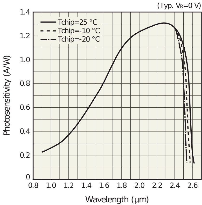
Figure 1: Photosensitivity of the Hamamatsu G12183 InGaAs-Photodiode. Source: Hamamatsu Photonics K.K., "InGaAs PIN photodiodes G12183 series", G12183-005 datasheet, Jan. 2021, page 3
